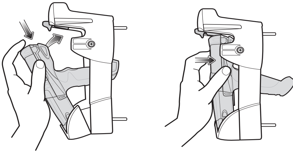
Figure 5-21 Insert MC9190-G into Forklift Cradle
