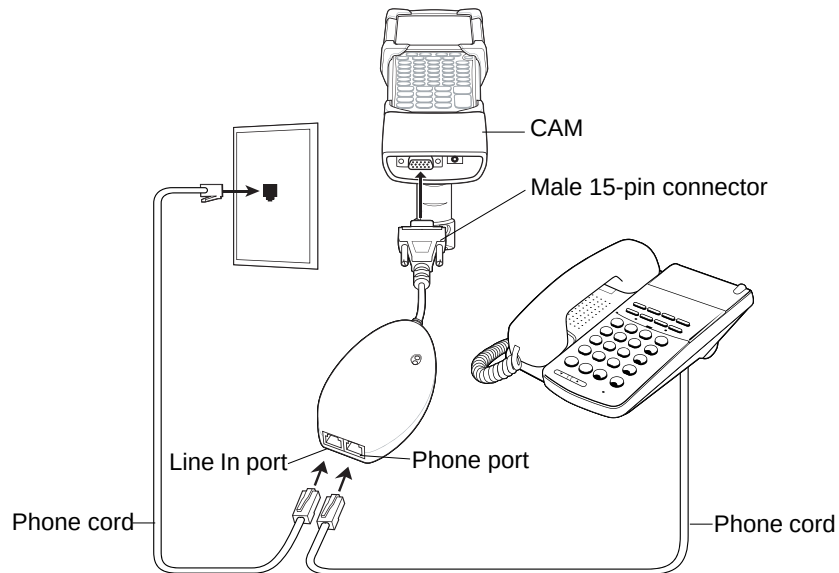
Figure 5-18 Modem Dangle Connection - MC9190-G
